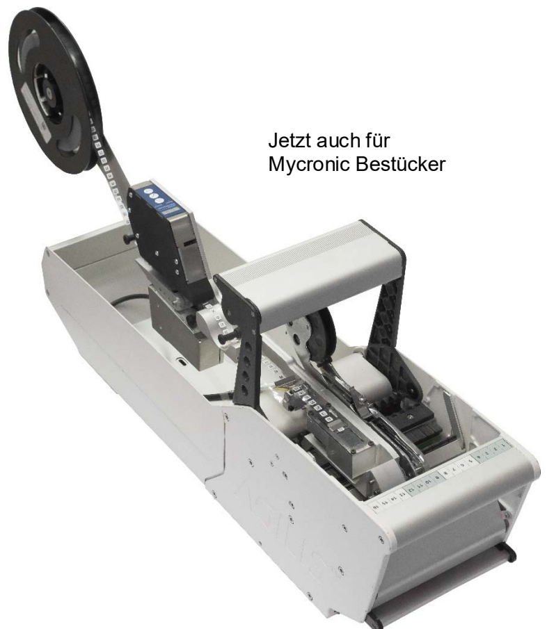
Standard Label Feeder ca. 60 mm
