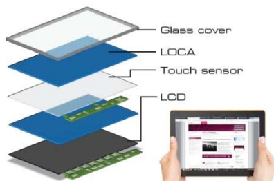
LOCA (Liquid Optical Clear Adhesive)
