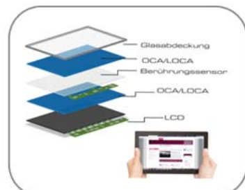
Optical Bonding
