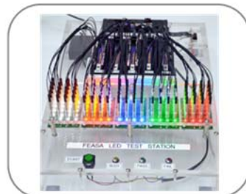
LED Analyse
