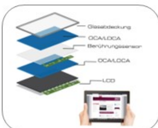
Optical Bonding
